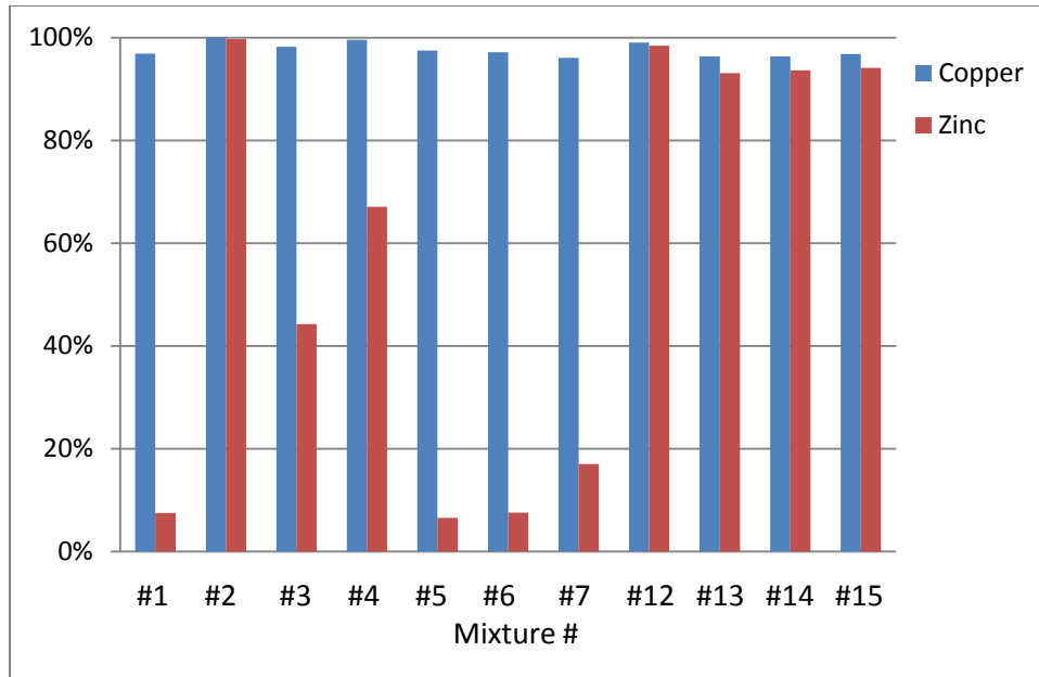
Figure B-1. Copper and zinc removal rates for biochar-based filtration media mixtures.
